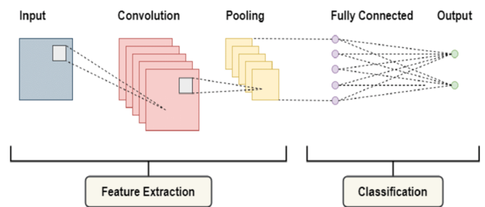
Figure 1. CNN architecture [2].
